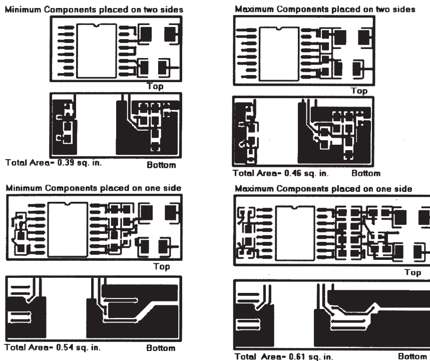
Figure 79. Recommended layout(s).
